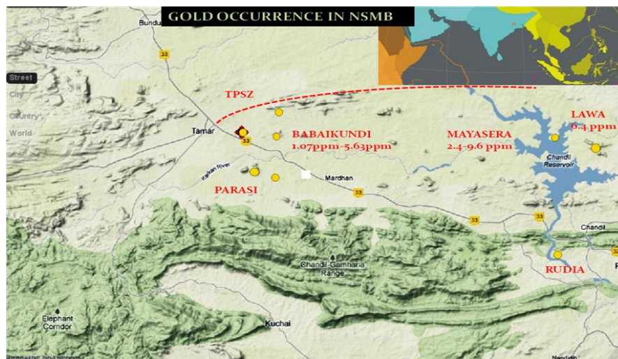
Figure 1: Gold Occurrences in NSMB, Jharkhand
