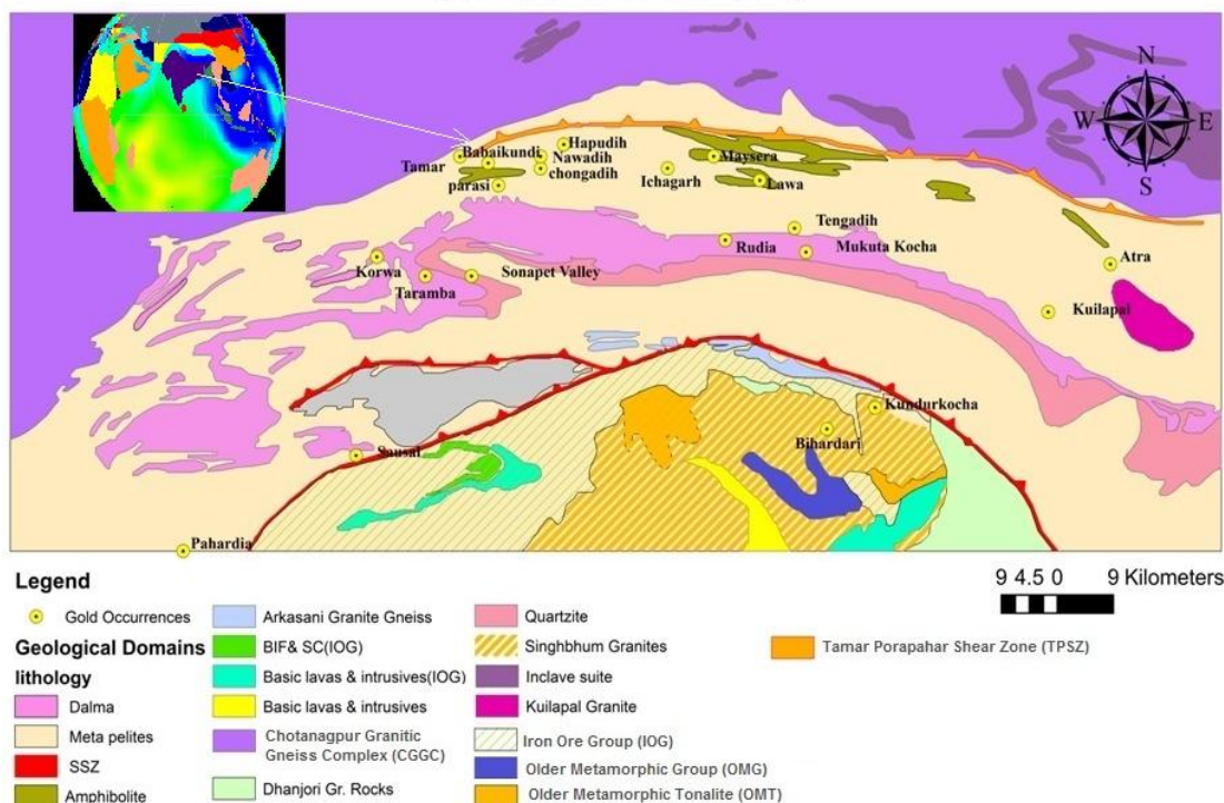
Figure 6: Geological Map of NSMB Showing the Gold Occurrences (Modified after S. Mahato & et al, 2008)
